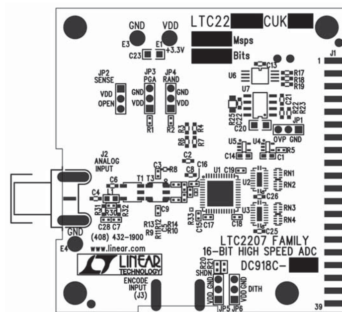
Silkscreen Top
